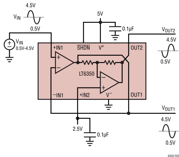
Figure 2. Basic Connections
