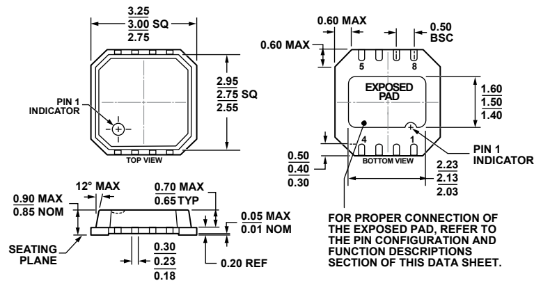
Figure 51. 8-Lead Lead Frame Chip Scale Package [LFCSP_VD] 3 mm × 3 mm Body, Very Thin, Dual Lead (CP-8-9)
