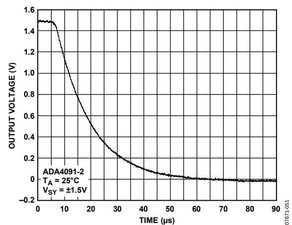
Figure 15. Positive Overload Recovery
