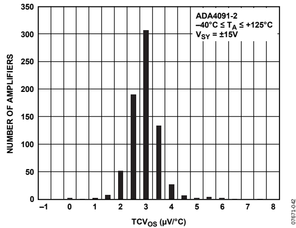
Figure 30. TCV_{OS} Distribution
