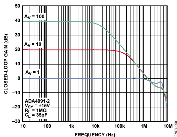
Figure 38. Closed-Loop Gain vs. Frequency
