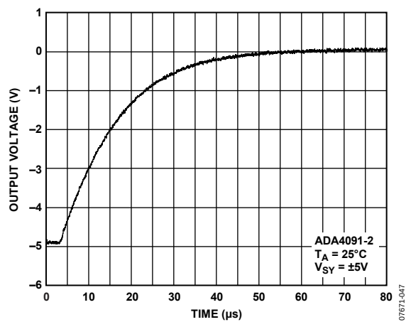
Figure 28. Negative Overload Recovery
