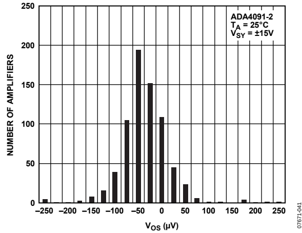
Figure 29. Input Offset Voltage Distribution
