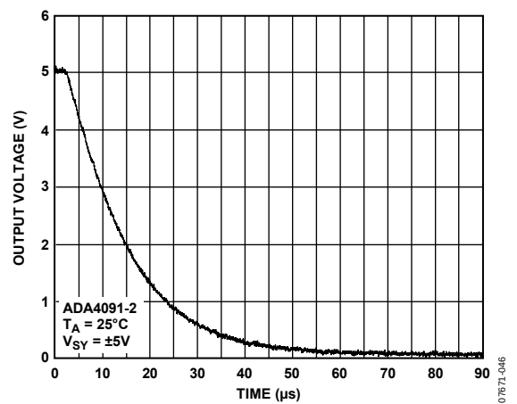
Figure 27. Positive Overload Recovery
