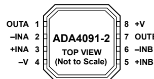
Figure 1. 8-Lead, Narrow-Body SOIC (R-8)
