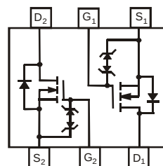
Top View Internal Schematic
