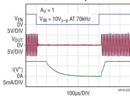
Enable/Disable Response
