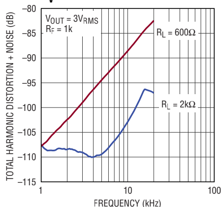
THD + Noise vs Frequency, A_V = -1
