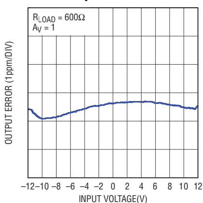
DC Linearity
