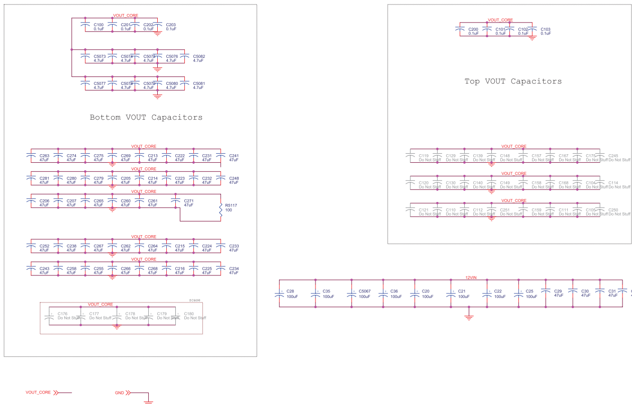
Figure 12. V_{IN} and V_{OUT} Capacitors Schematic
