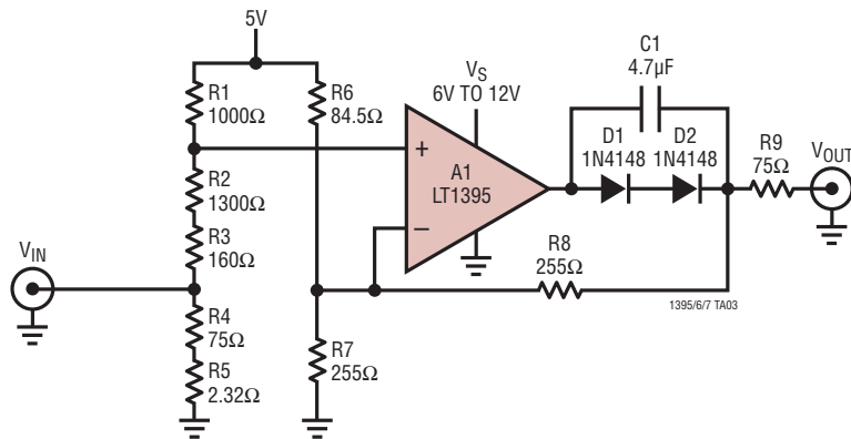
Figure 6. Single Supply RGB Video Amplifier (1 of 4 Channels)
