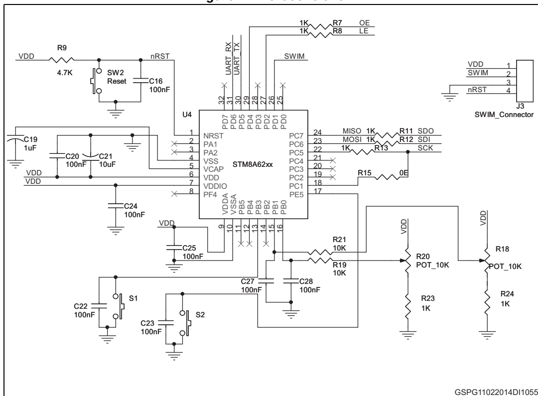
Figure 2. Microcontroller
