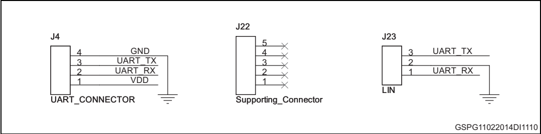
Figure 5. Connector
