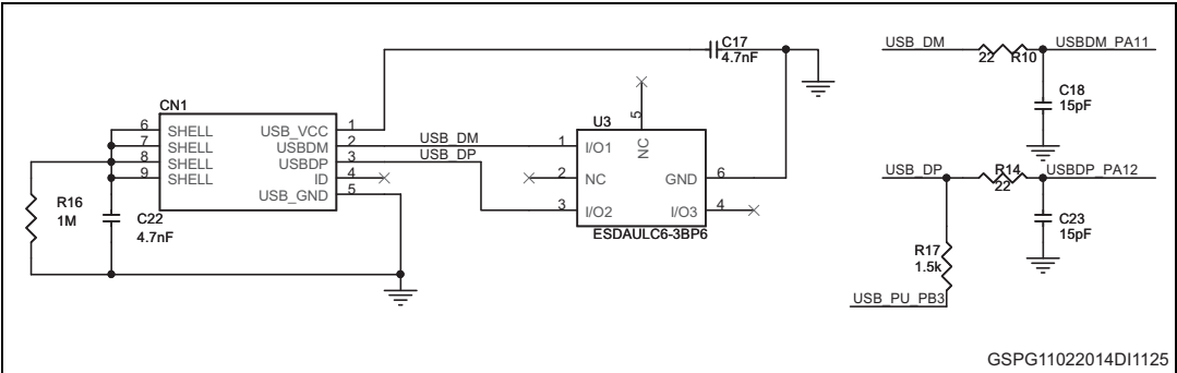
Figure 8. USB section
