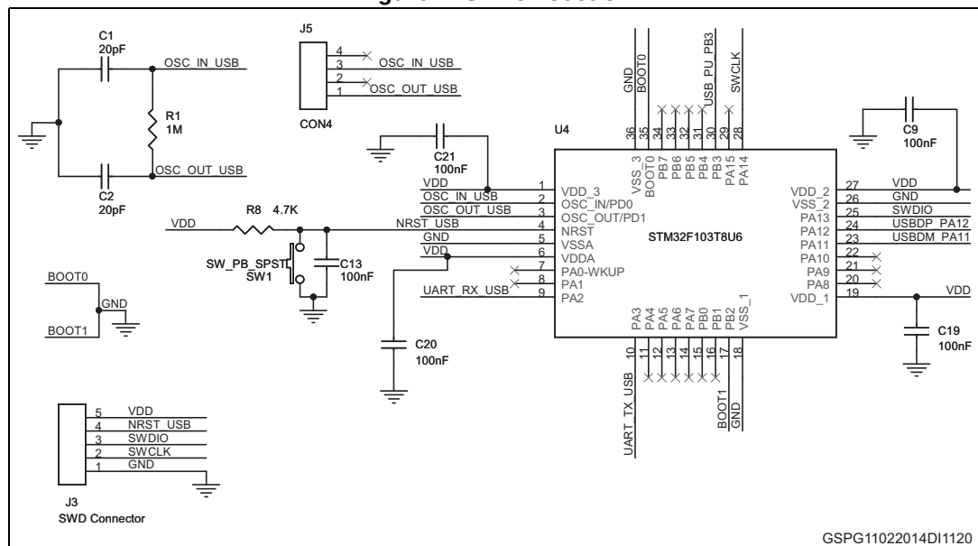
Figure 7. STM32 section
