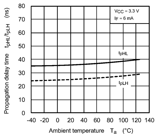
Fig. 12.2.9 t_{pHL}/t_{pLH} - T_a
