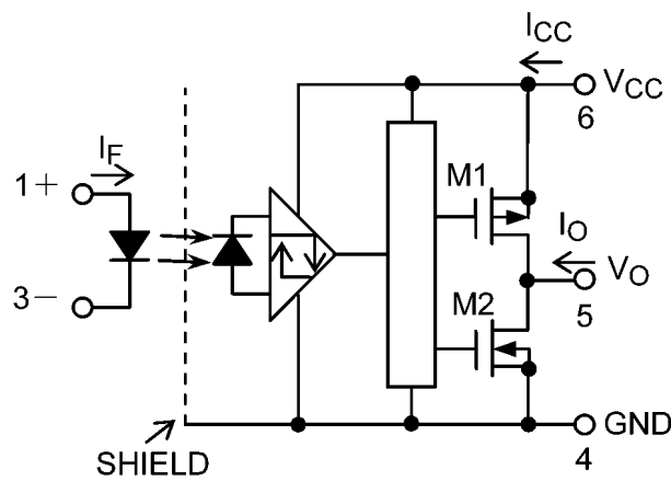
Fig. 5.1 Internal Circuit
