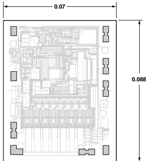
TOP VIEW (CIRCUIT SIDE)
