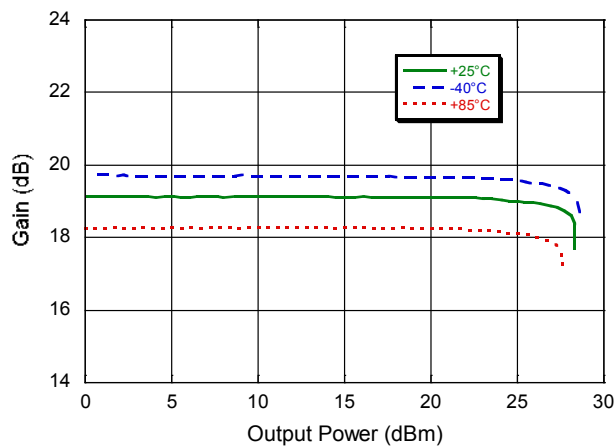
P1dB @ 250 MHz
