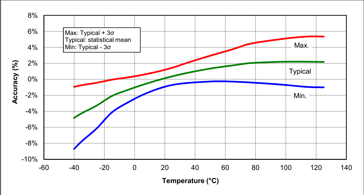
FIGURE 26-52: HFINTOSC ACCURACY OVER TEMPERATURE, 2.3V ≤ VDD ≤ 5.5V
