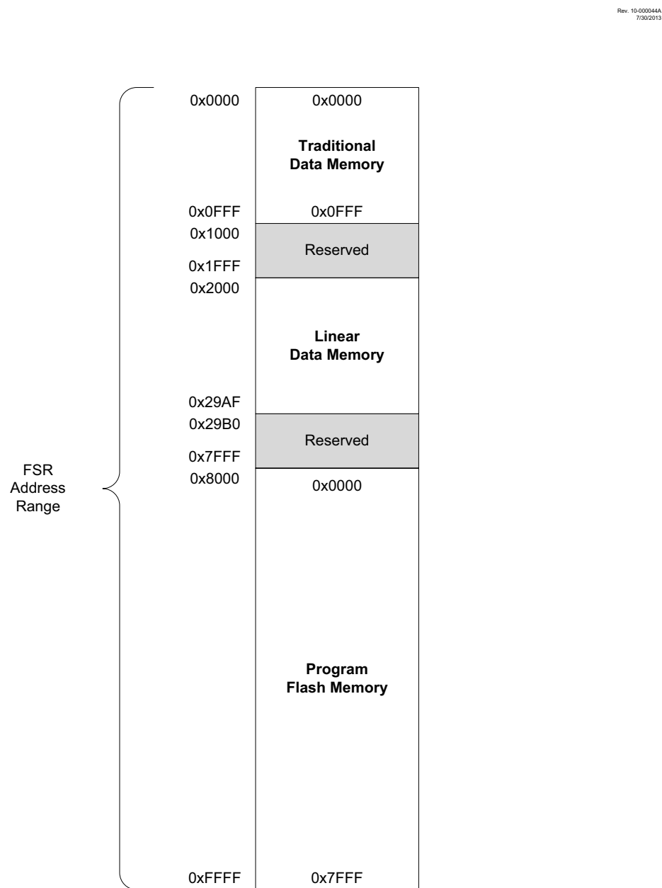
FIGURE 3-8: INDIRECT ADDRESSING
