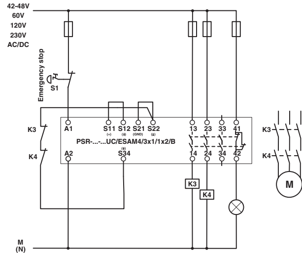
Figure 5 Emergency stop with automatic start
