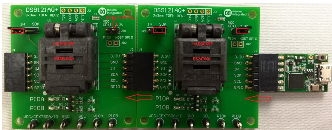
Figure 9. Orientation of the DS28E83 and DS2476 in the Burn-In Socket
