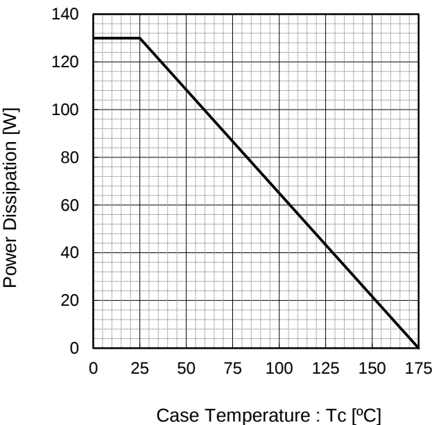
Fig.6 Power Dissipation
