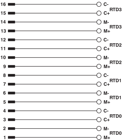
Circuit diagram
