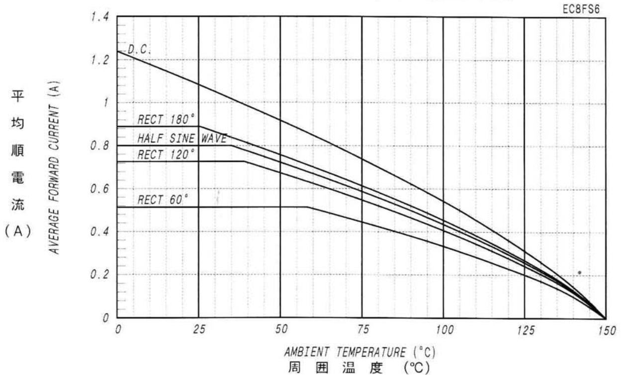
平均順電流一周圍溫度定格 AVERAGE FORWARD CURRENT VS. AMBIENT TEMPERATURE
