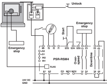
Circuit diagram
