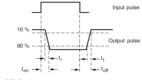
Fig. 4 - Test Circuit and Waveforms
