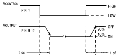
OUTPUT TURN-ON AND TURN-OFF TIMING
