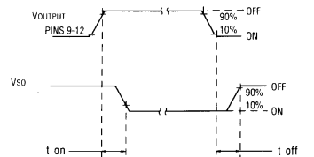
STATUS TURN-ON AND TURN-OFF TIMING
