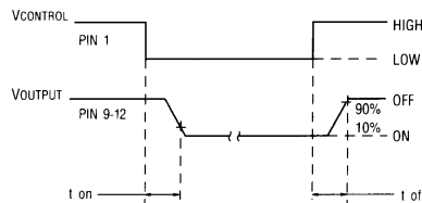
OUTPUT TURN-ON AND TURN-OFF TIMING (A) FIGURE 5
