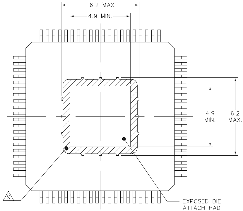
VIEW J-J
