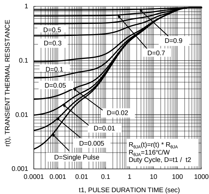
Figure 6. Transient Thermal Resistance
