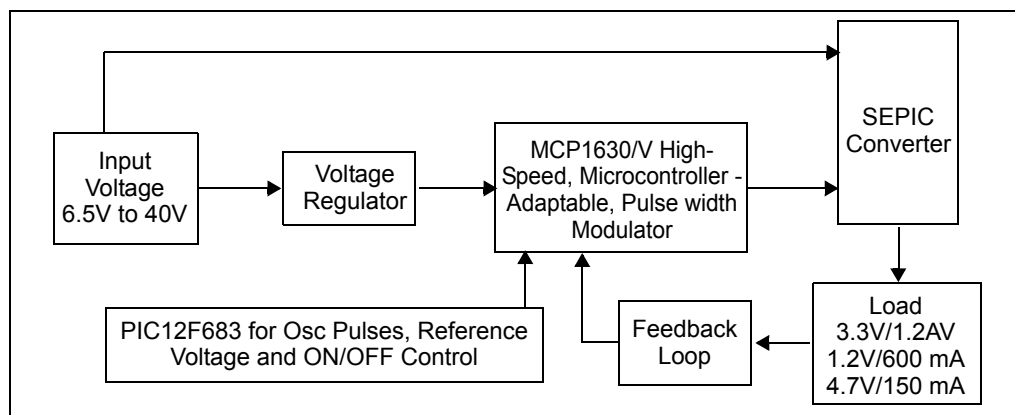
FIGURE 1-1: MCP1630 Automotive Input Triple Output Converter Demo Board Block Diagram.
