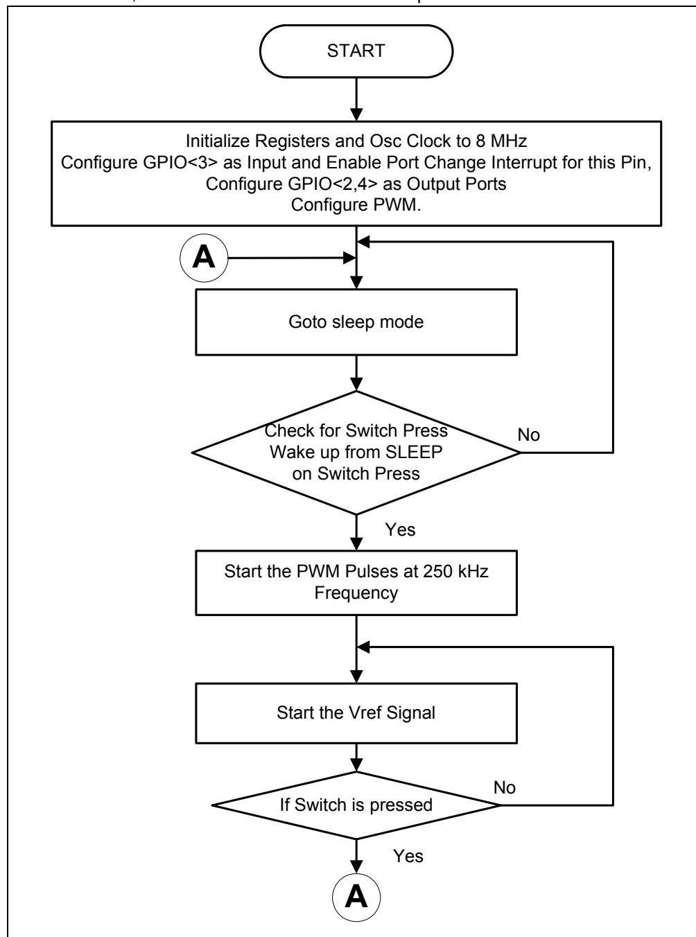
FIGURE C-1: Firmware Flowchart.
