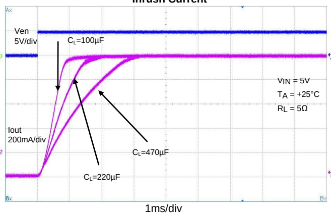
Inrush Current
