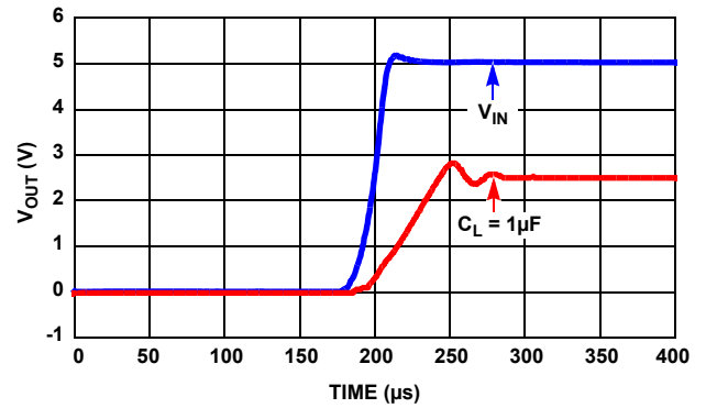
FIGURE 27. TURN-ON TIME WITH 1 \mu F
