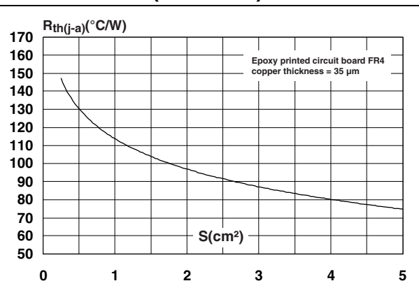
Figure 14. Thermal resistance junction to ambient versus copper surface under anode (SMBflat-3L)
