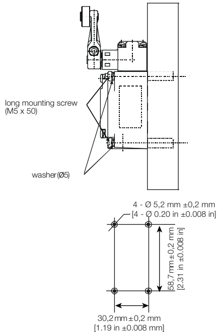
Figure 16. Surface Mount
