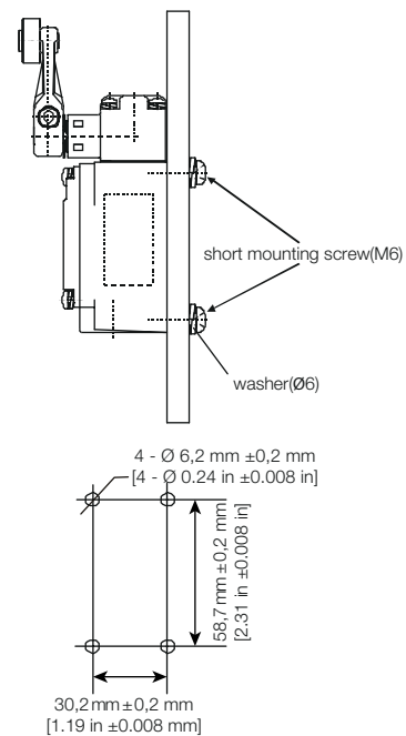
Figure 18. Rear Mount
