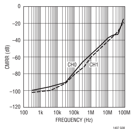
Figure 3. CMRR vs Frequency
