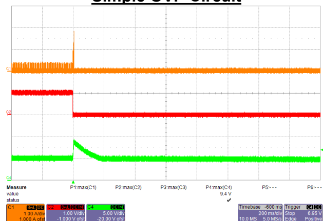
Figure 42 – Output Overvoltage (Open Loop), 90 VAC, No-Load Upper: I DRAIN , 1 A / div. Middle: Opto Diode Voltage, 1 V / div. Lower: V OUT , 5 V, 200 ms / div. OVP at 9.4 V
