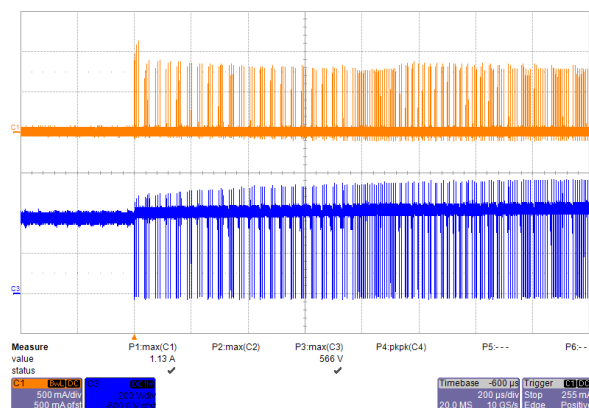
Figure 23 – Start-up Profile, 265 VAC, Full Load Upper: I_{DRAIN} , 0.5 A / div. Lower: V_{DRAIN} , 200 V, 200 \mu s / div.
