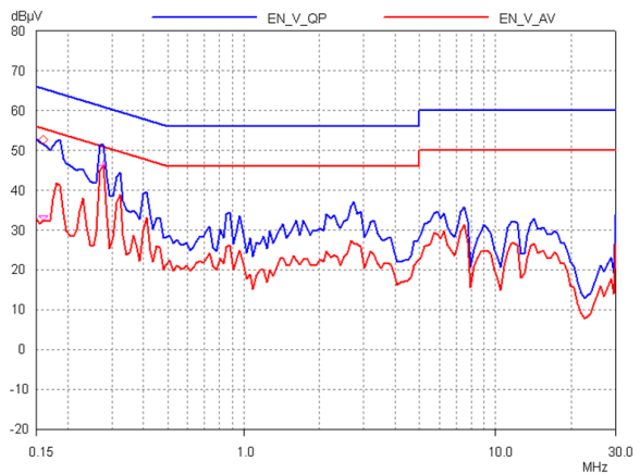
Figure 53 – 230 VAC, Neutral.
