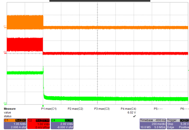
Figure 47 – Output Overvoltage (Open Loop), 90 VAC, Full Load Upper: I_{DRAIN} , 1 A / div Middle: Opto Diode Voltage, 1 V / div Lower: V_{OUT} , 2 V, 200 ms / div. OVP at 6.02 V
