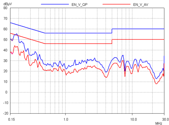
Figure 51 – 115 VAC, Neutral.
