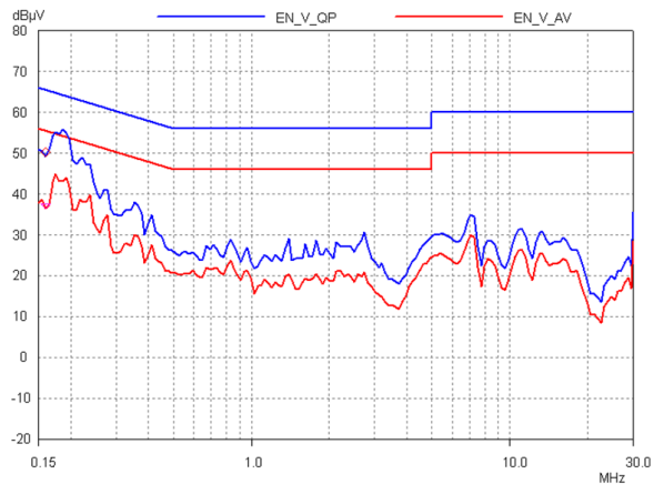
Figure 50 – 115 VAC, Line.
