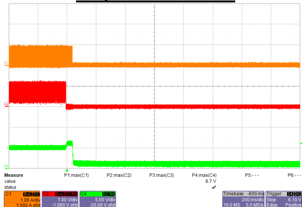
Figure 46 – Output Overvoltage (Open Loop), 90 VAC, Full Load Upper: I_{DRAIN} , 1 A / div Middle: Opto Diode Voltage, 1 V / div Lower: V_{OUT} , 5 V, 200 ms / div. OVP at 6.7 V
