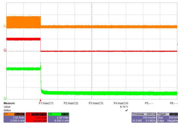
Figure 49 – Output Overvoltage (Open Loop), 265 VAC, Full Load Upper: I_{DRAIN} , 1 A / div. Middle: Opto Diode Voltage, 1 V / div. Lower: V_{OUT} , 2 V, 200 ms / div. OVP at 6.14 V
