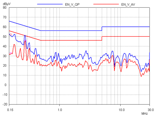
Figure 52 – 230 VAC, Line.
