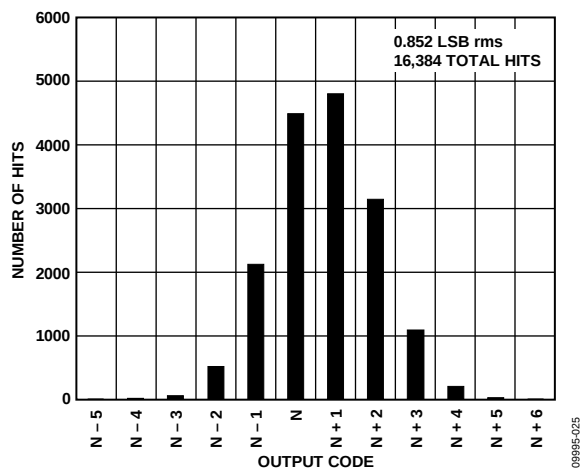
Figure 27. AD9642-210 Grounded Input Histogram, f_s = 210 MSPS
