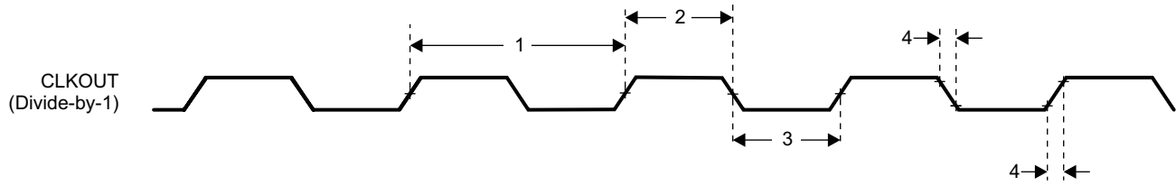
Figure 7-10. CLKOUT Timing
