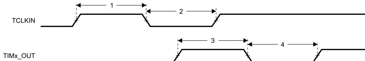
Figure 8-88. Timer Timing
