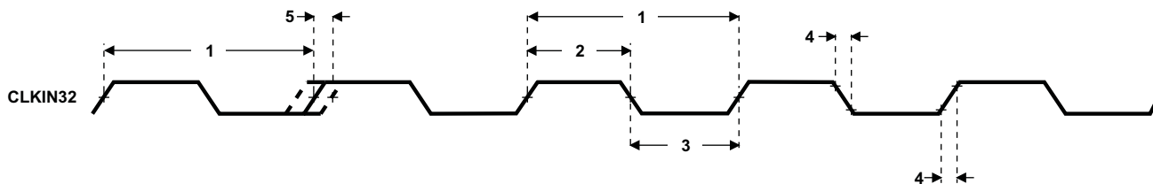
Figure 7-7. CLKIN32 Timing
