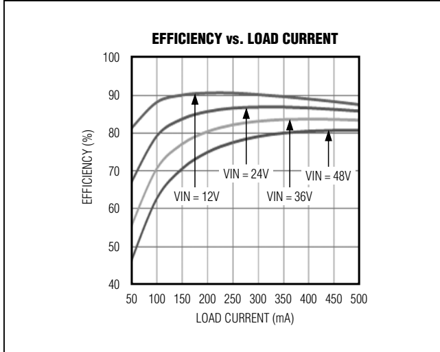
Figure 2. MAX17501H Efficiency
