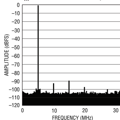
LTC2258-14: 8k Point FFT, f_{IN} = 5\text{MHz} , -1\text{dBFS} , 65Msps
