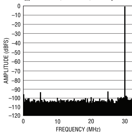
LTC2258-14: 8k Point FFT, f_{IN} = 30\text{MHz} , -1\text{dBFS} , 65Msps
