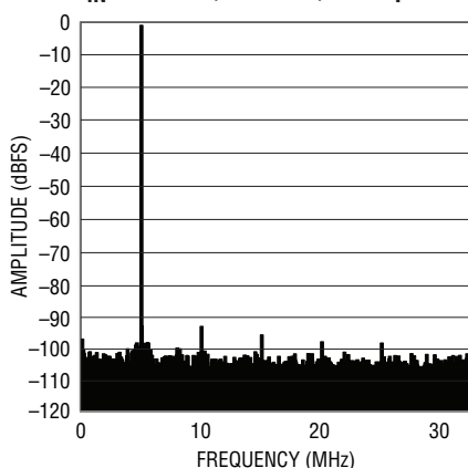
LTC2258-14: 8k Point FFT, f_{IN} = 70\text{MHz} , -1\text{dBFS} , 65Msps
