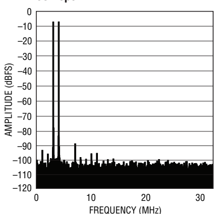
LTC2258-14: 8k Point 2-Tone FFT, f_{IN} = 68\text{MHz} , 69MHz, -1\text{dBFS} , 65Msps
