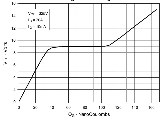
Fig. 8. Gate Charge
