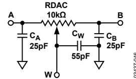
Figure 46. Circuit Simulation Model for RDAC = 10 kΩ
