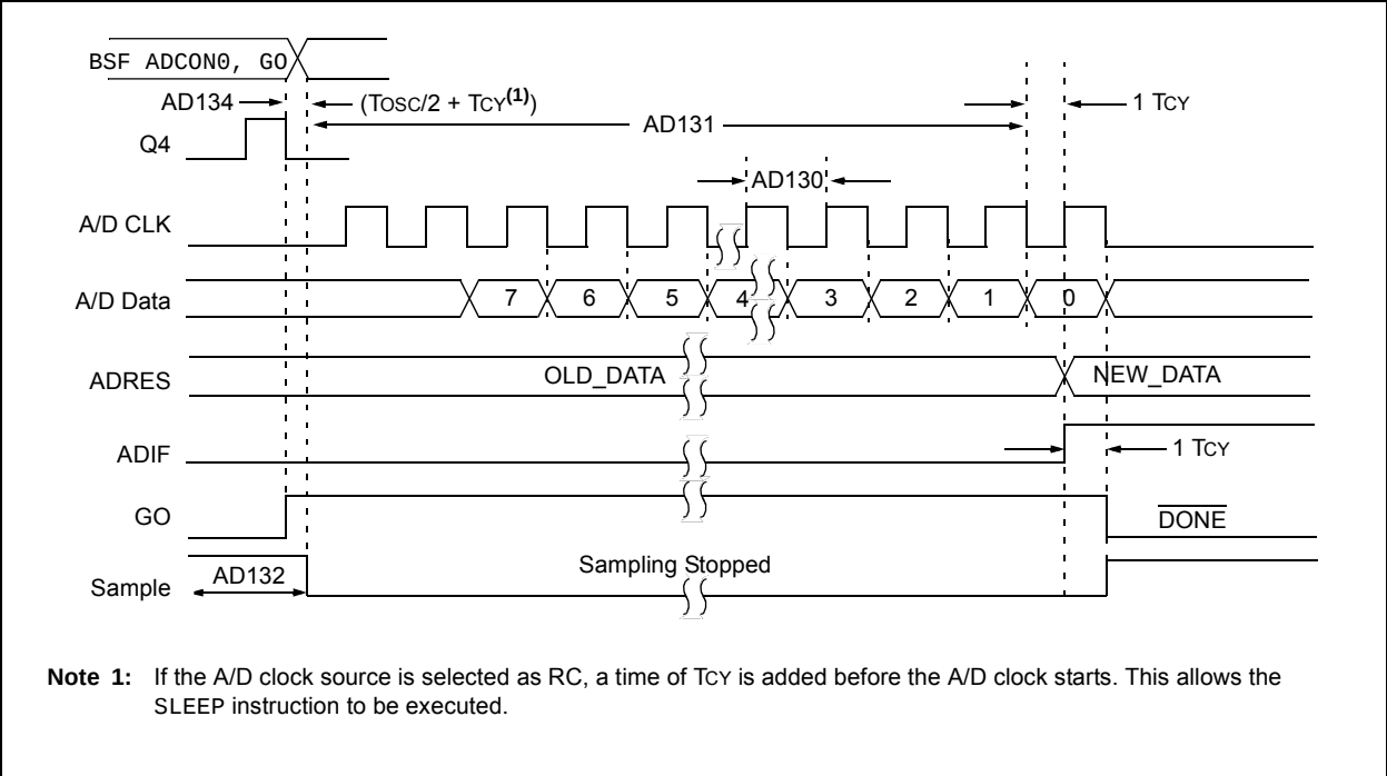
FIGURE 30-13: PIC16(L)F1824/8 A/D CONVERSION TIMING (SLEEP MODE)
