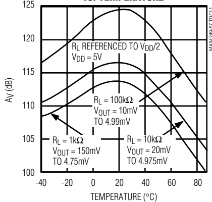
LARGE-SIGNAL VOLTAGE GAIN vs. TEMPERATURE
