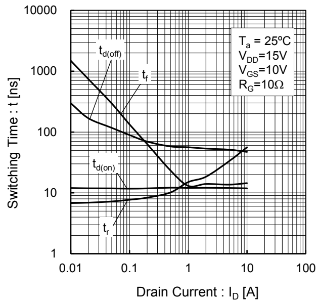
Fig.19 Switching Characteristics
