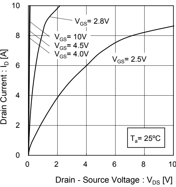
Fig.6 Typical Output Characteristics(II)
