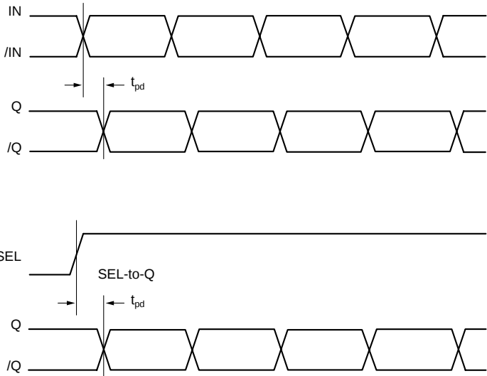
Figure 2. Timing Diagram
