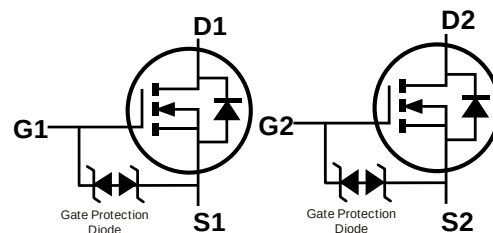
Equivalent Circuit
