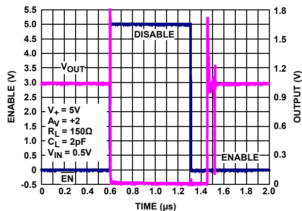
FIGURE 12. ENABLE/DISABLE TIMING
