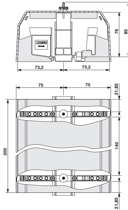
Dimensioned drawing
