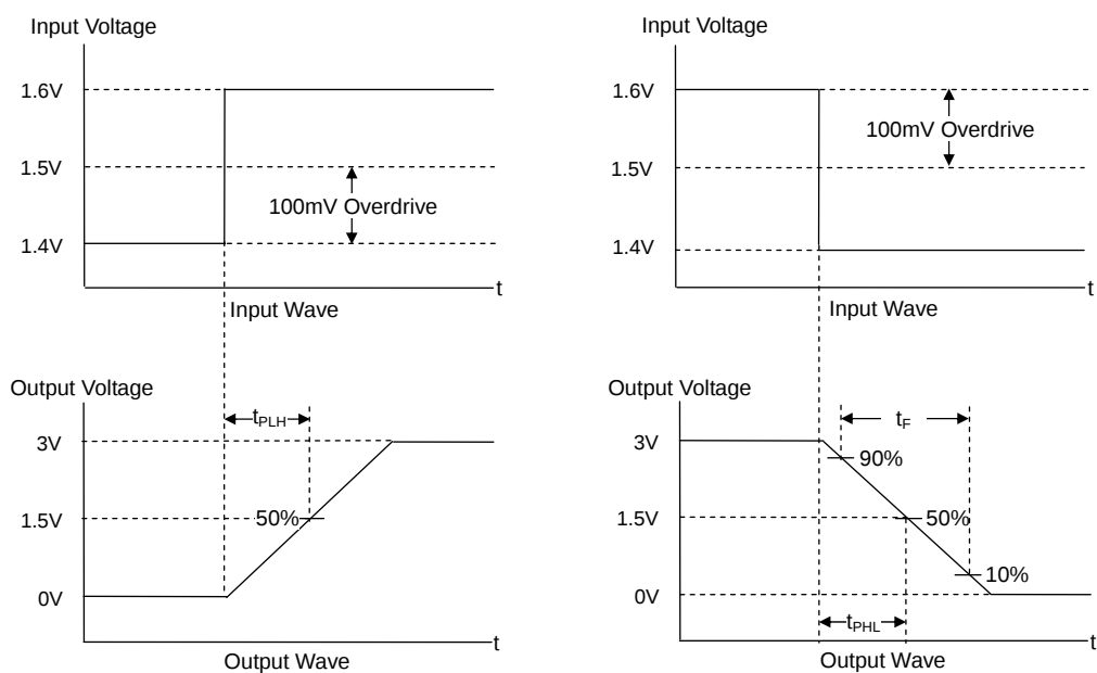
Figure 43. Response Time Input and Output Wave
