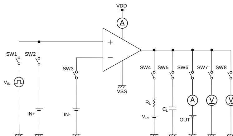
Figure 42. Test Circuit 2 (One channel only)
