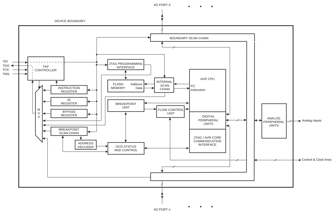
Figure 83. Block Diagram
