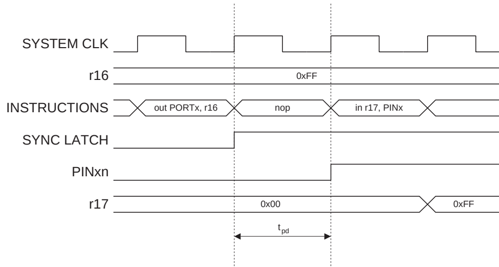
Figure 31. Synchronization when Reading a Software Assigned Pin Value
