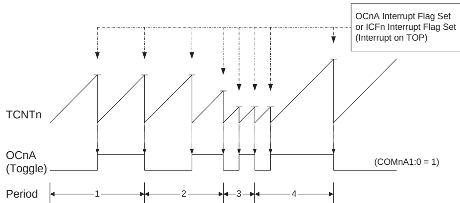
Figure 51. CTC Mode, Timing Diagram
