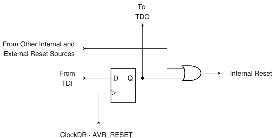
Figure 86. Reset Register
