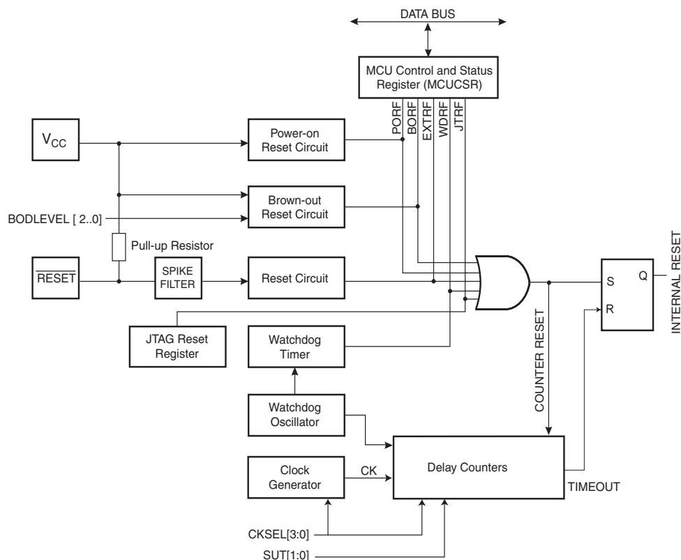
Figure 21. Reset Logic
